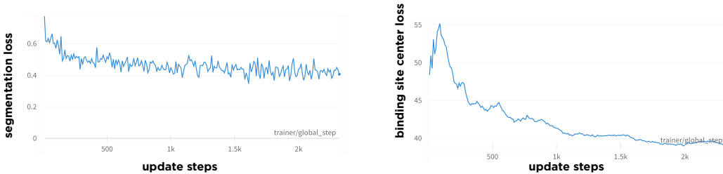
Figure L1: Training curves of a VN-EGNN during development. The model was trained only using segmentation loss, i.e. Dice loss. Left: Learning curve depicting the segmentation loss during training. Right: Learning curve depicting the positional binding site center point loss, which was not explicitly optimized for this experiment. Despite only being trained to minimize the segmentation loss, the virtual nodes converged towards the known binding sites centers.
